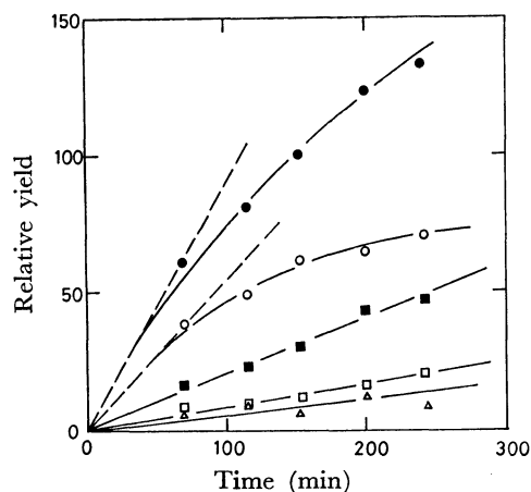
Fig. 2. Relative yields of cresols (●), benzaldehyde (○), m -nitrotoluene (■), p -nitrotoluene (□), and benzyl nitrate (△) vs. irradiation time in the photo-oxidation of toluene- \text{HNO}_2 -air system.
