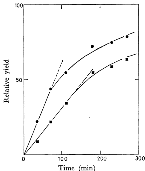
Fig. 1. Relative yields of phenol (●) and nitrobenzene (■) vs. irradiation time in the photo-oxidation of benzene- \text{HNO}_2 -air system.
