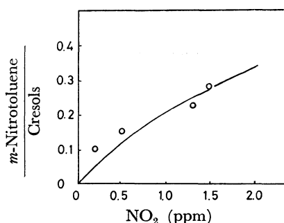
Fig. 3. Yields of m -nitrotoluene relative to cresols as a function of initial concentration of \text{NO}_2 in the photo-oxidation of toluene- \text{HNO}_2 -air system.
